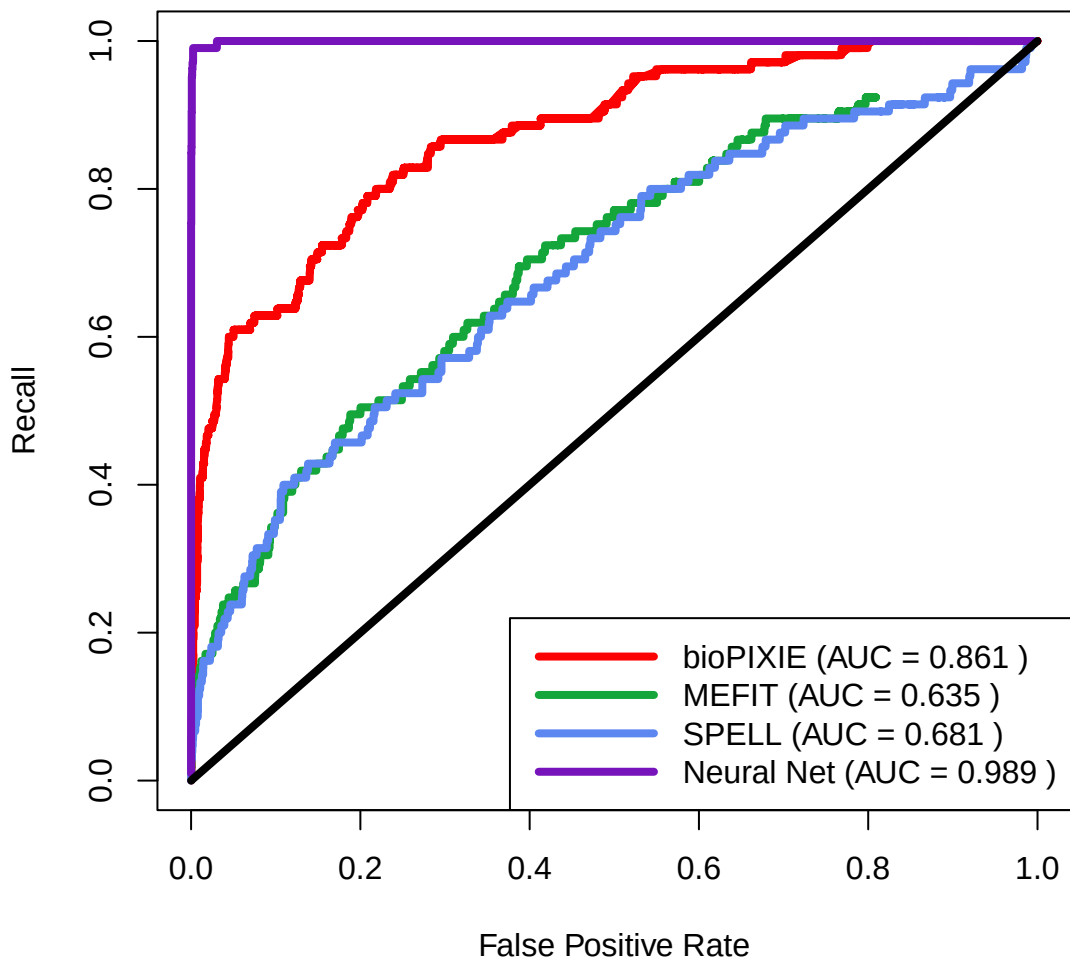
Ensemble Comparison 430x20x1
